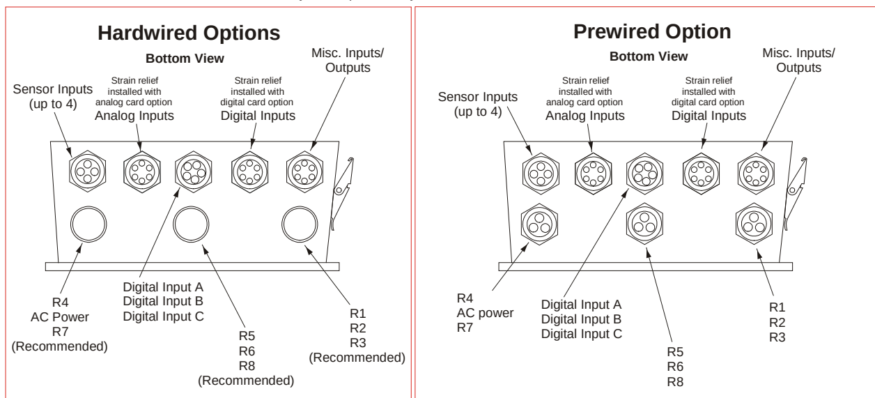
Figure 2: Conduit/Wiring Configuration
