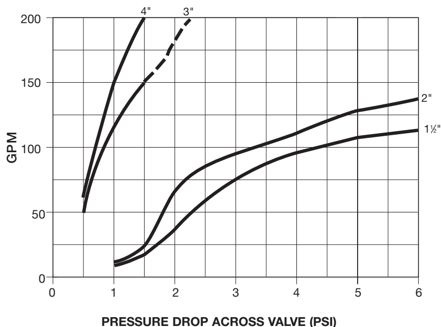
CKS CHECK VALVE FLOW CHART Tested with City Water Under Laboratory Conditions
