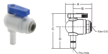
VTEU - Valve Tube Elbow Union
