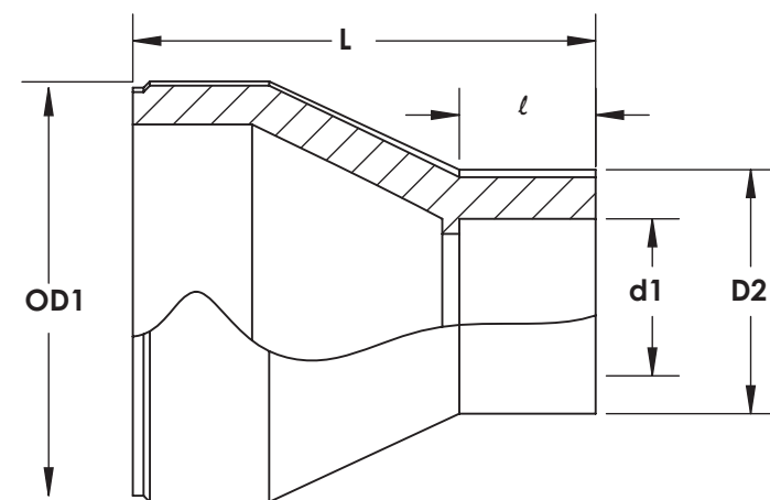
Concentric Reducer
