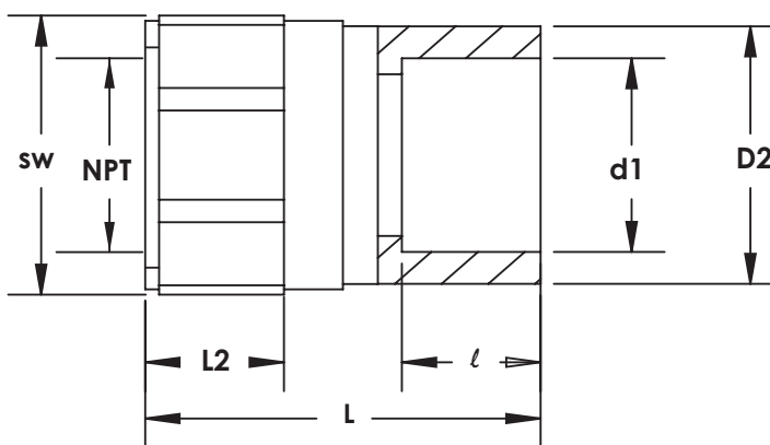
Female Adapter
