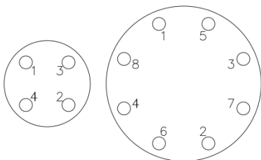
Fig. 1: Flange Bolt Torque Sequence
