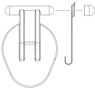
Fig. 2A: Disc, spring, and end cap (unassembled)
