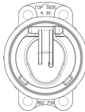
Fig. 2B: Disc, spring, and end cap inside body
