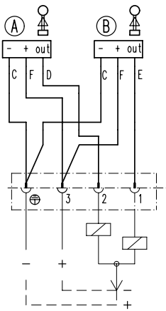
Circuit diagram
