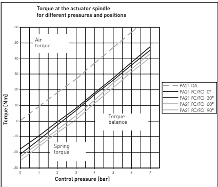
PA21 Torque characteristics
