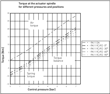
PA 11 Torque characteristics
