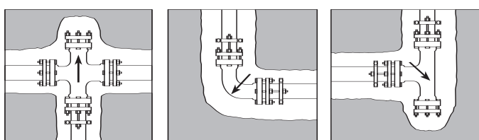
Thru line connection, cross used as tee Direction change, elbow Direction change, tee used as elbow
