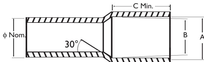
GF Harvel Belled-End Pipe Dimensions
