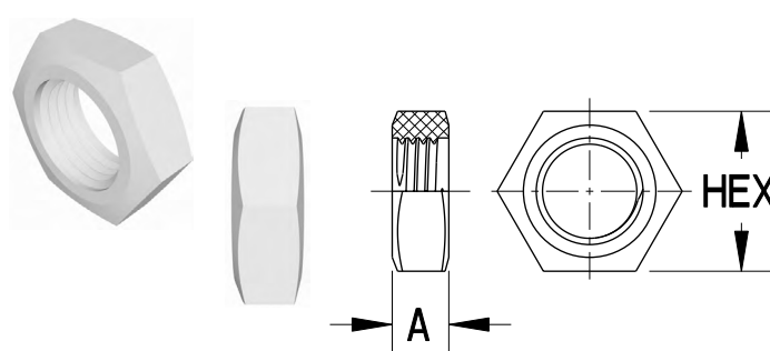
Furon® PVDF Panel Nut
