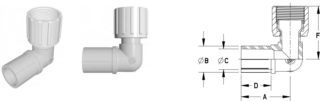
Furon® ETAFF Elbow Tube Adapter Female Flare
