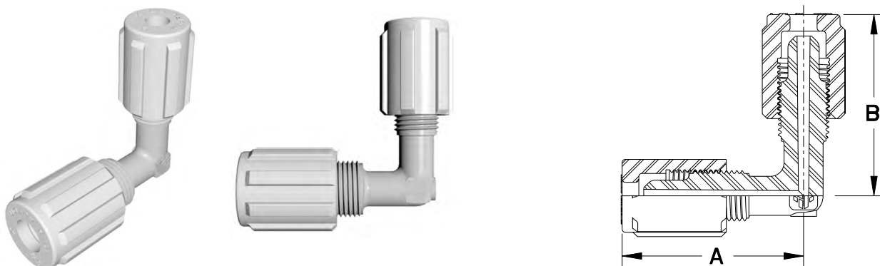
Furon® UE Union Elbow
