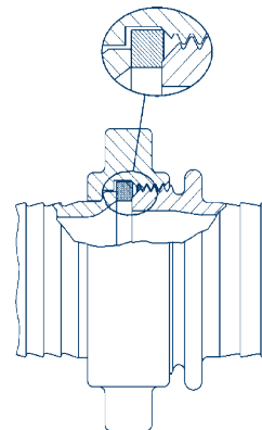
washer seal
