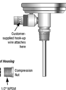
Type TT.30 w/RTD terminal block
