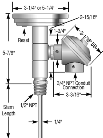
Type TT.30 w/enclosure head
