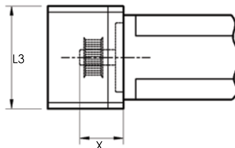
Side View (Carriage Up)
