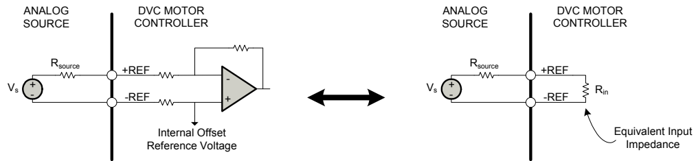
FIGURE 3.4 Analog Source and Drive Input
