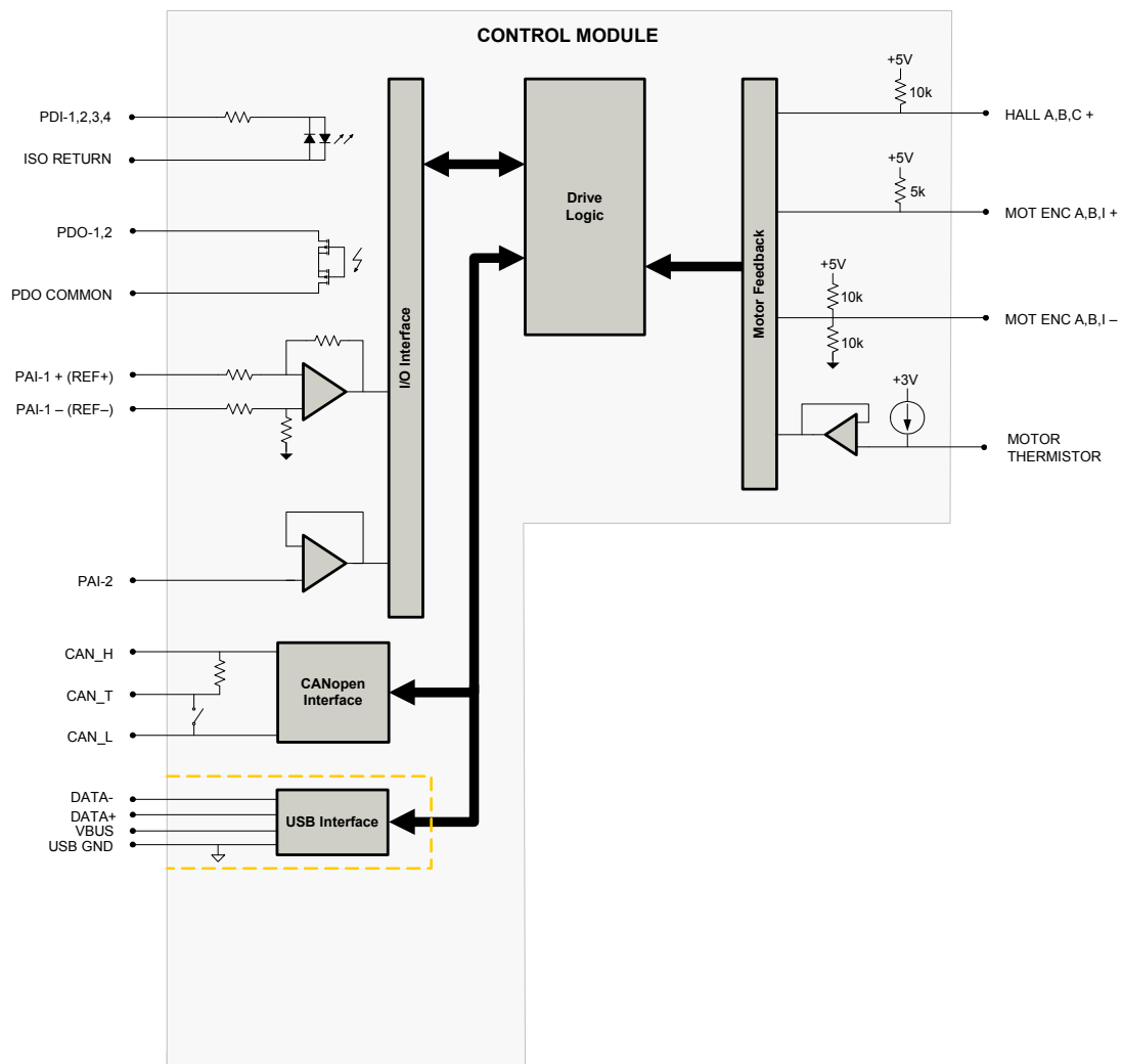
FIGURE 2.2 DVC Control Module
