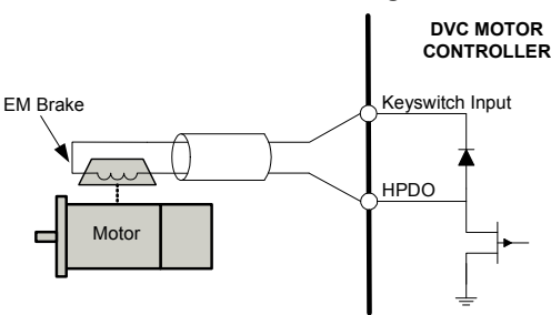
FIGURE 4.5 HPDO Electromagnetic Brake Example
