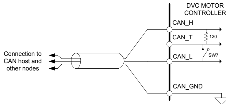
FIGURE 4.13 CANopen Interface
