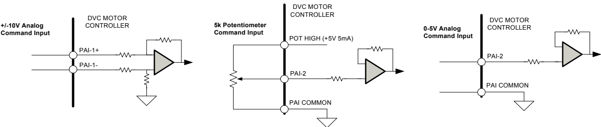
FIGURE 4.4 Programmable Analog I/O Commands
