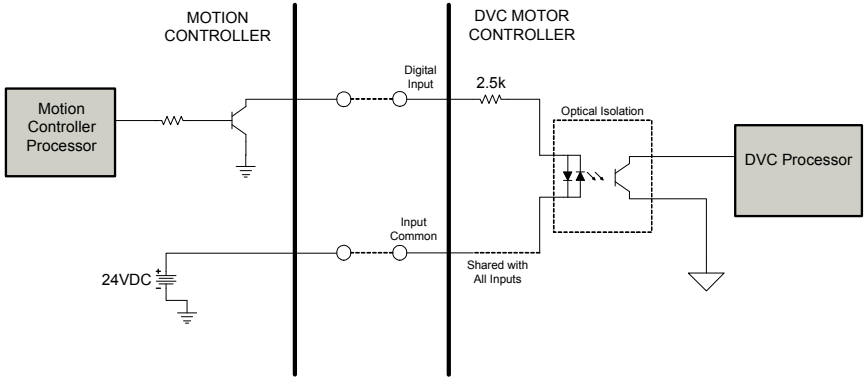
FIGURE 4.2 24VDC Isolated Digital Input configured as a sourcing input.
