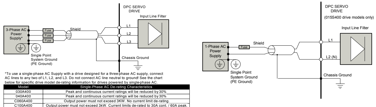
FIGURE 4.17 AC Power Module Supply Wiring
