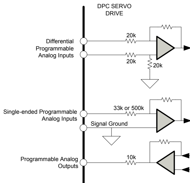
FIGURE 4.9 Programmable Analog I/O
