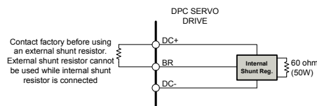
FIGURE 4.27 030A800 Power Module External Shunt Resistor Connection
