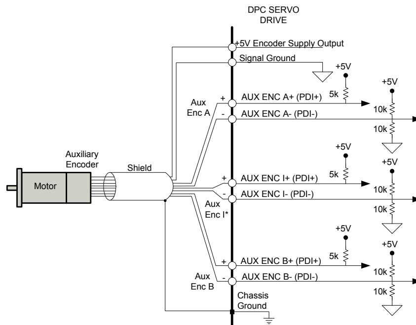
FIGURE 4.7 Auxiliary Encoder Input Connections
