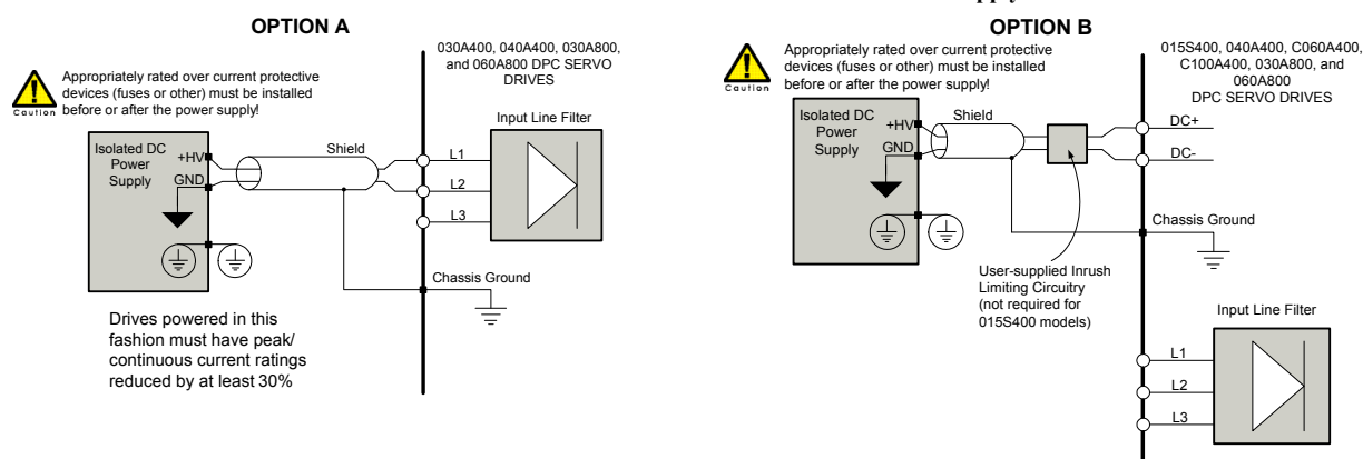
FIGURE 4.18 AC Power Modules with DC Power Supply
