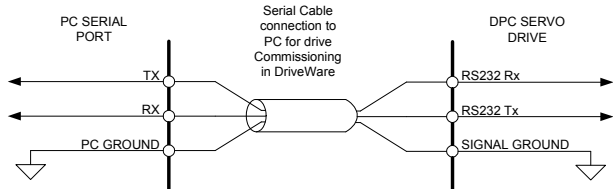
FIGURE 4.30 RS-232 Interface
