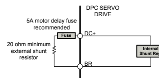
FIGURE 4.26 C100A400 Power Module External Shunt Resistor Connection
