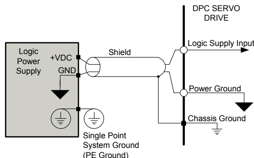
FIGURE 4.21 DC Power Module Logic Power Supply Inputs
