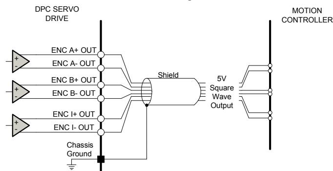
FIGURE 4.8 Encoder Output Connections
