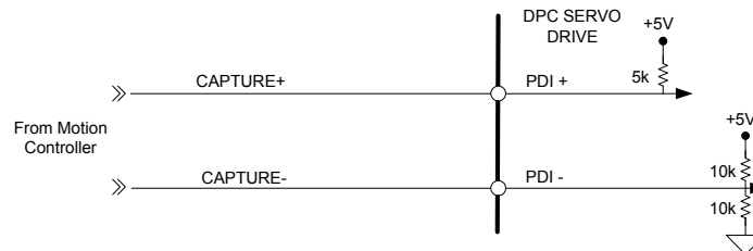
FIGURE 4.6 High-Speed Capture Input Connections
