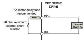
FIGURE 4.25 C060A400 Power Module External Shunt Resistor Connection
