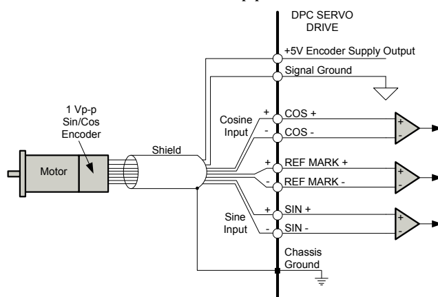
FIGURE 4.11 1 Vp-p Sin/Cos Encoder
