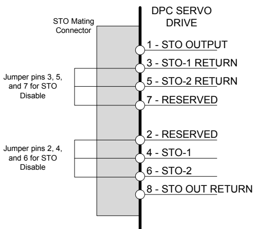
FIGURE 4.23 STO Disable Connections
