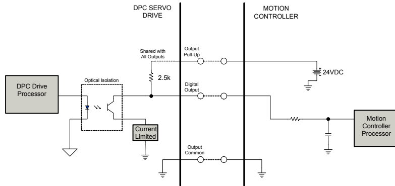
FIGURE 4.3 24VDC Isolated Digital Output configured as a sourcing output.
