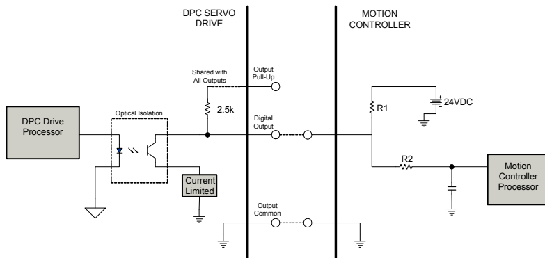
FIGURE 4.4 24VDC Isolated Digital Output configured as a sinking output.
