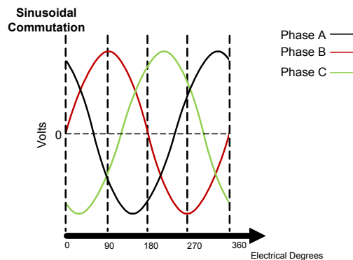
FIGURE 4.31 Sinusoidal Commutation Motor Phase Currents
