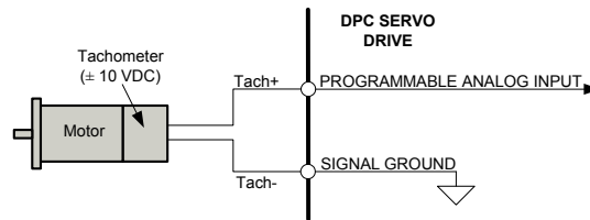
FIGURE 4.14 Tachometer Input Connections
