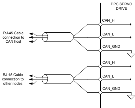
FIGURE 4.29 CANopen Interface
