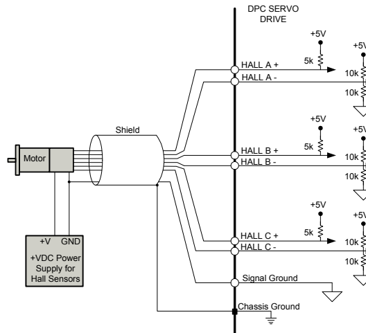
FIGURE 4.15 Hall Sensor Input Connections
