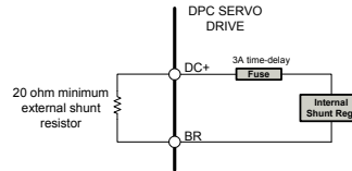
FIGURE 4.24 030A400 Power Module External Shunt Resistor Connection
