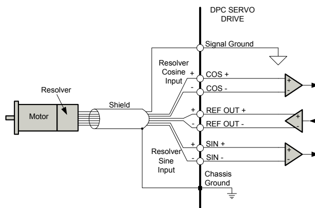
FIGURE 4.13 Resolver Input Connections
