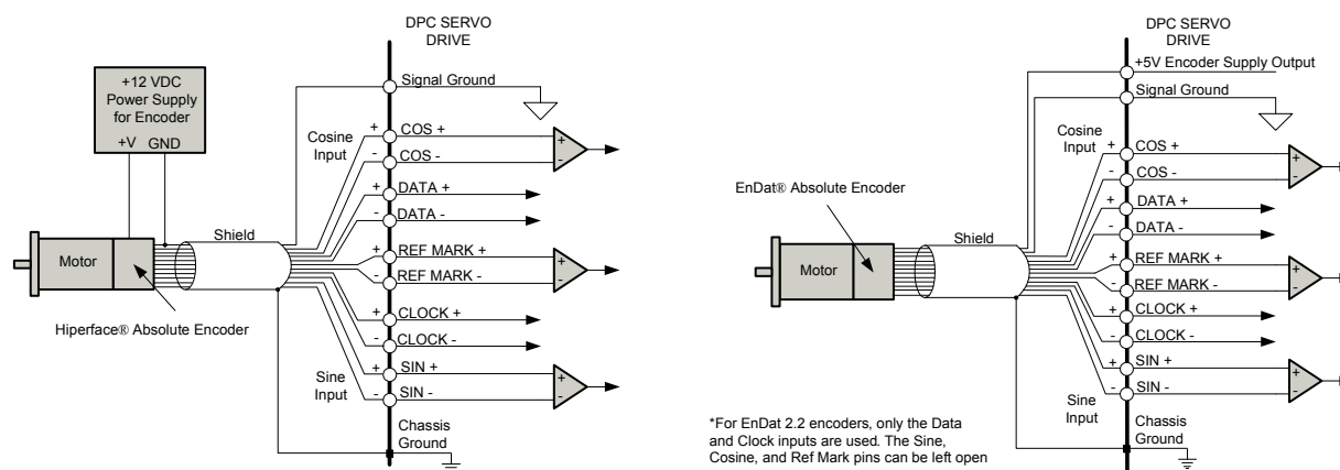
FIGURE 4.10 Absolute Encoder Connections
