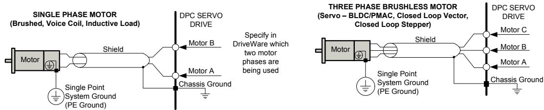
FIGURE 4.16 Motor Power Output Wiring
