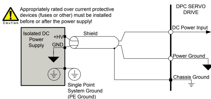
FIGURE 4.19 DC Power Module Supply Wiring
