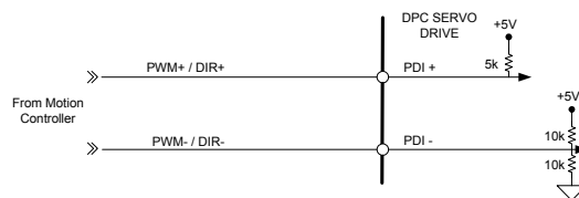
FIGURE 4.5 PWM and Direction Input Connections
