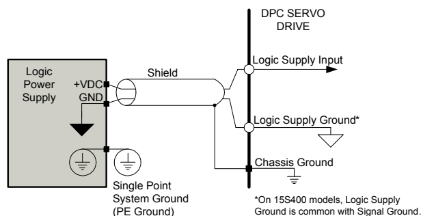
FIGURE 4.20 AC Power Module Logic Power Supply Inputs
